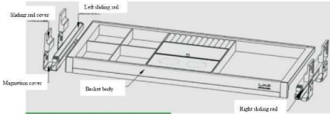
Picture 1: multiply functions box 600/800/900/1000
